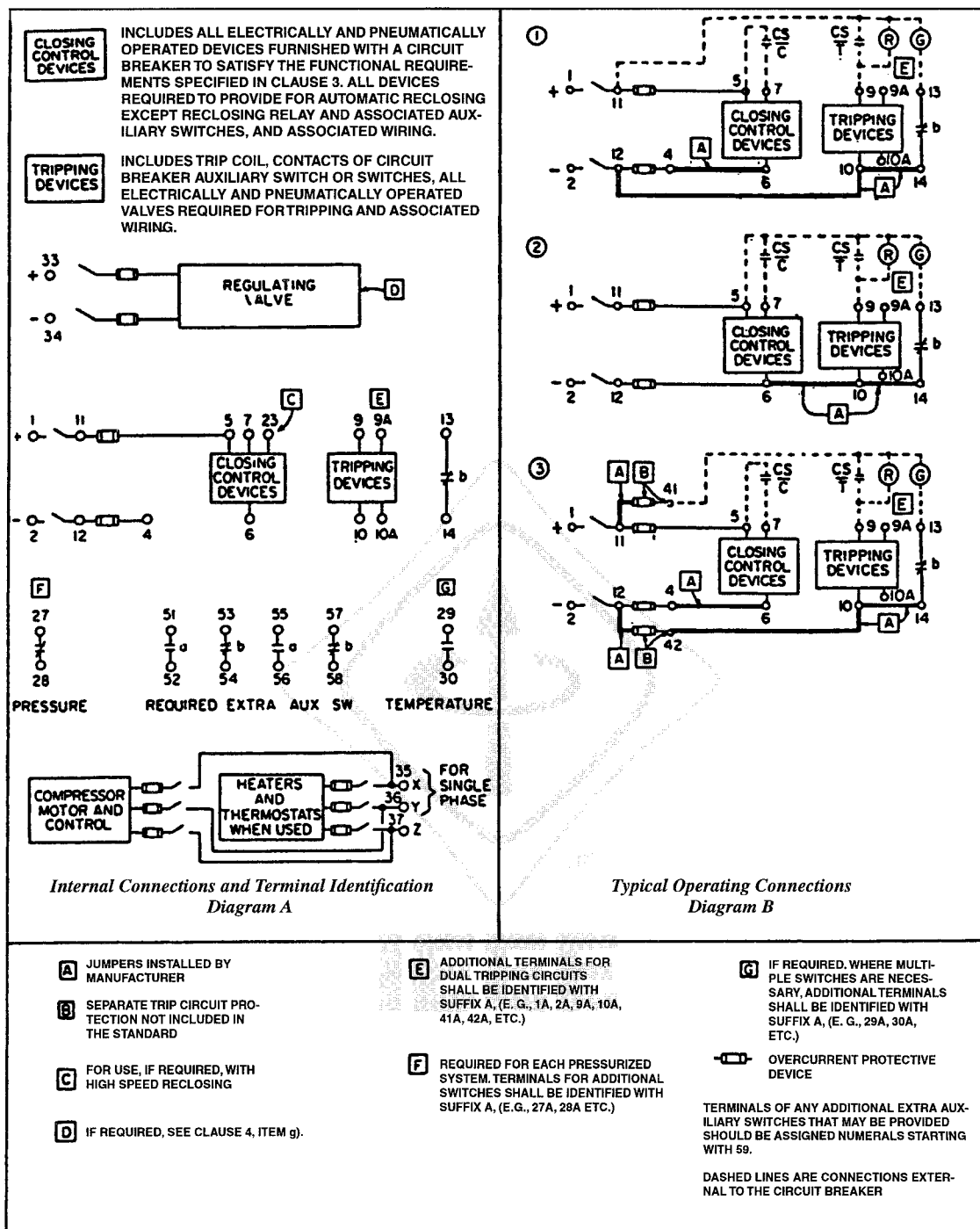
Figure 8—Pneumatically—or hydraulically—operated circuit breaker NOT intended for use in metal-clad switchgear, where —The closing control is dc —The tripping control is dc
