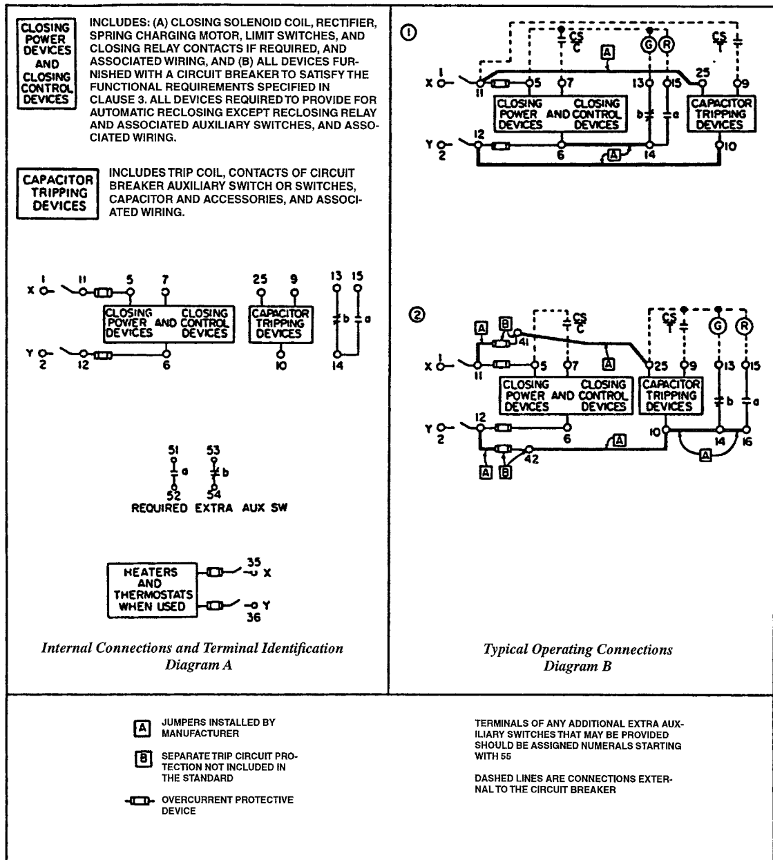
Figure 3—Circuit breaker intended for use in metal-clad switchgear, where
