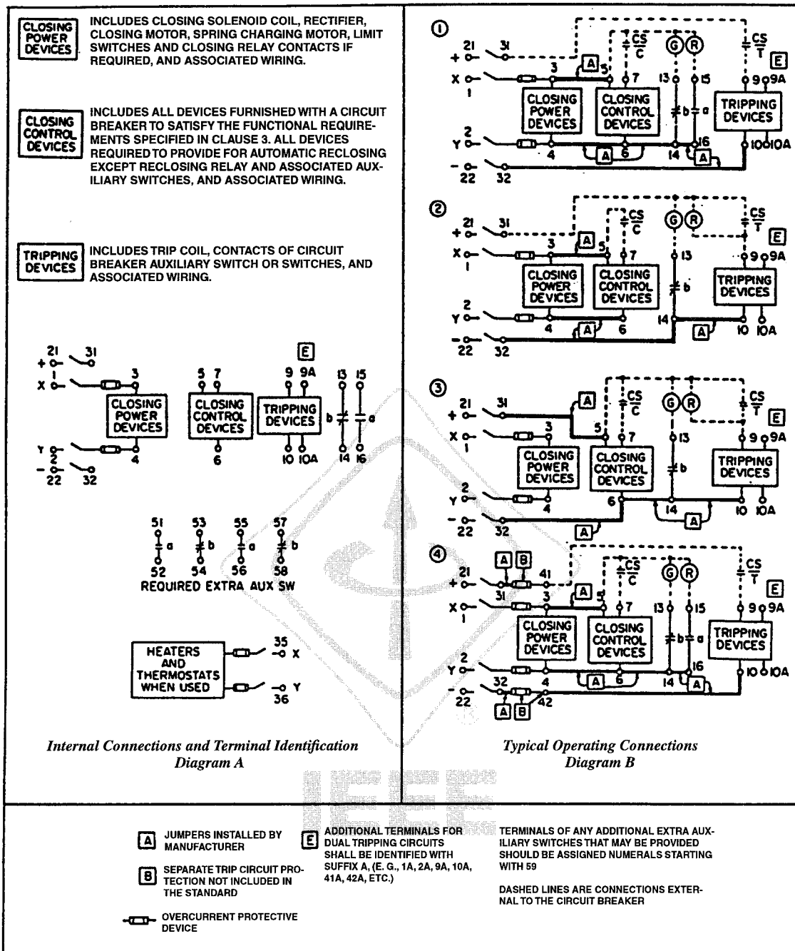
Figure 6—Circuit breaker NOT intended for use in metal-clad switchgear, where —The closing power is ac —The closing control is ac or dc —The tripping control is dc
